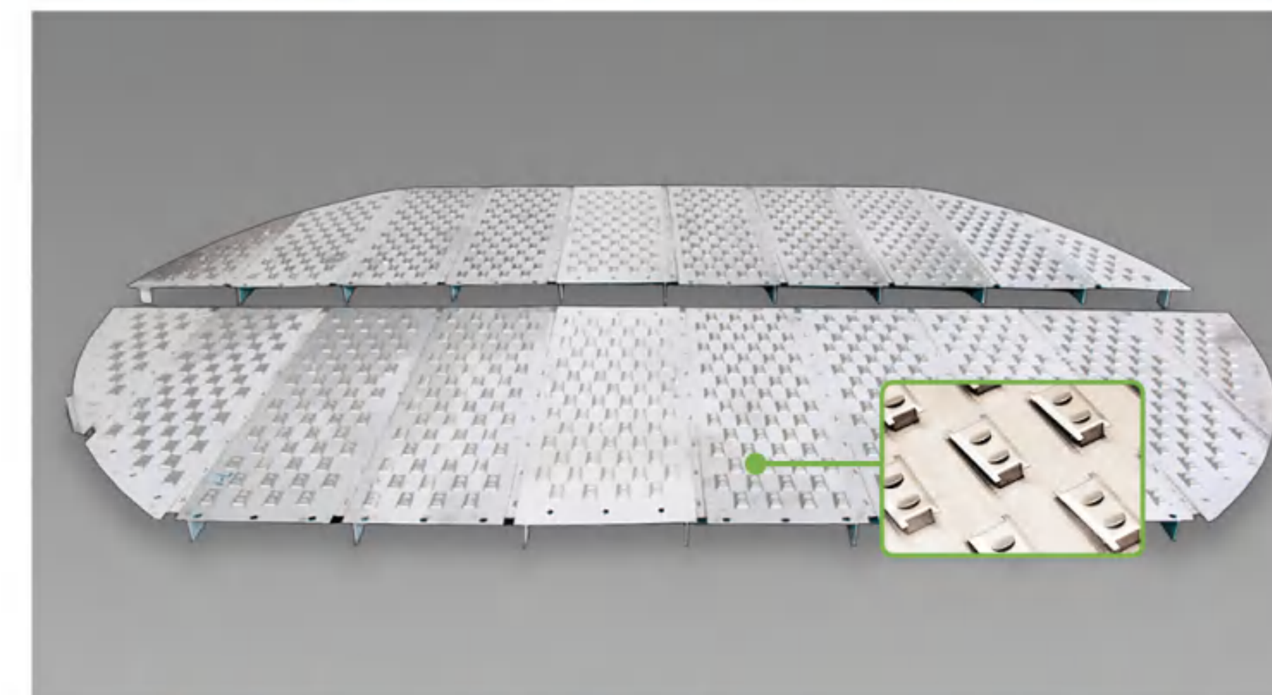
The Trapezoid Guide Floating Valve Tray
