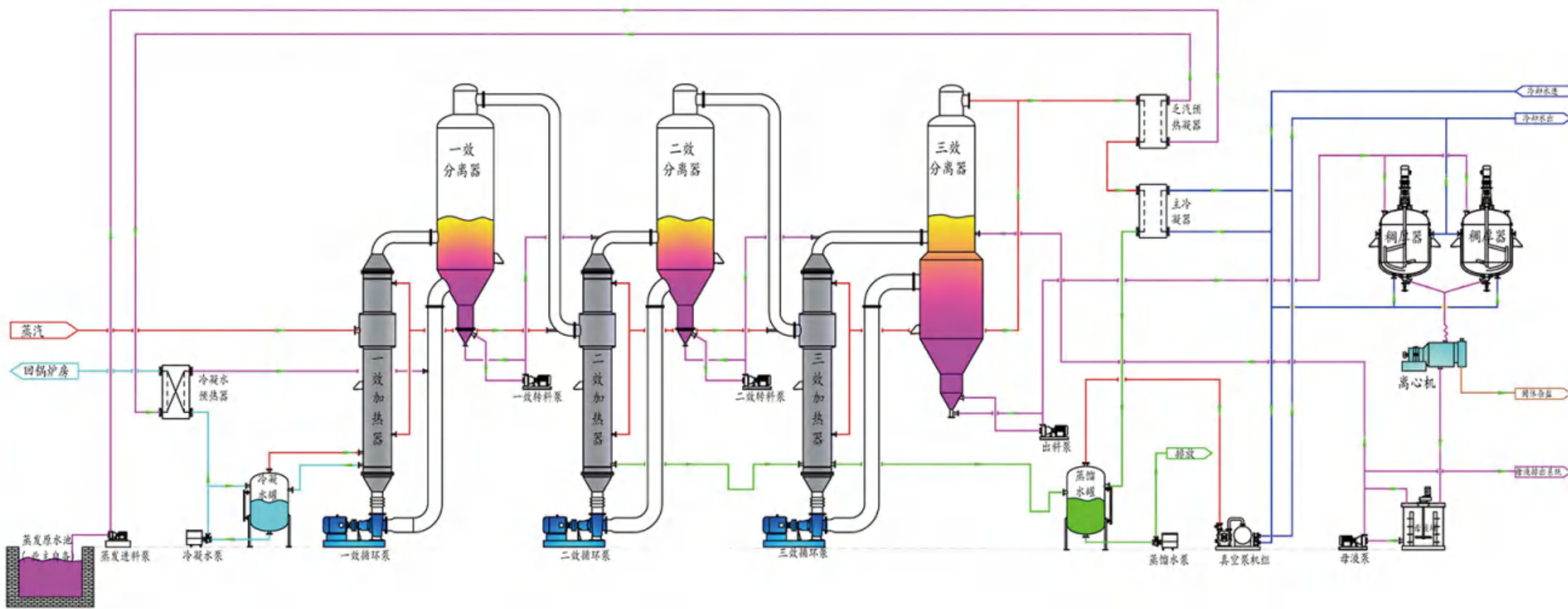
Three effects forced circulation PID
