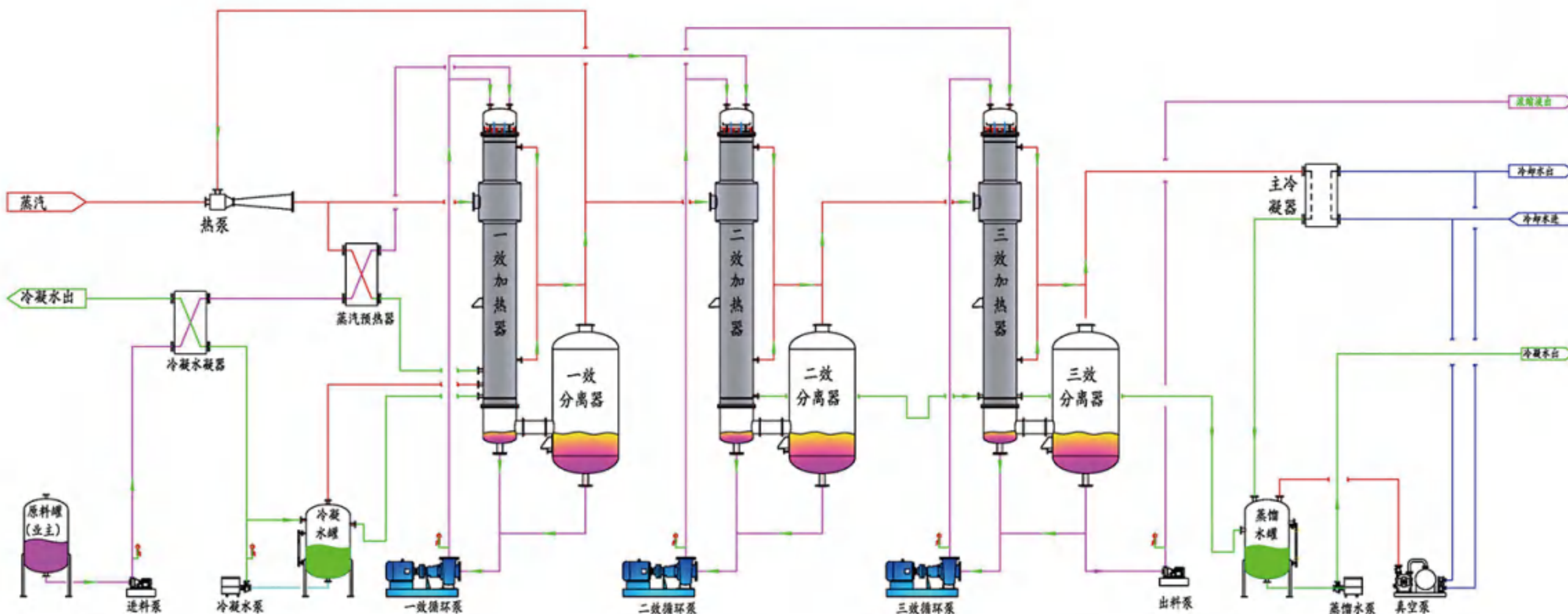
TVR three effects evaporation system PID
